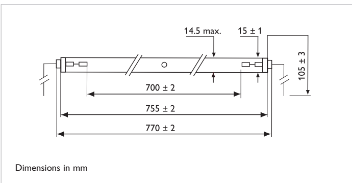
Philips HTK 7/60
