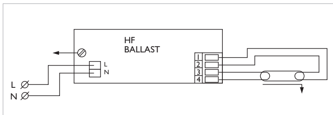
Circuit 6
