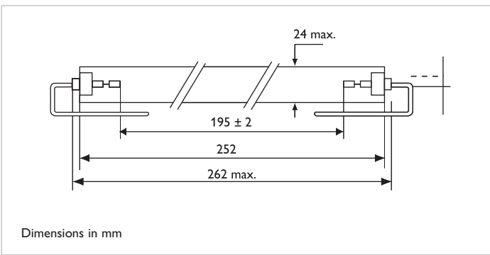
Philips HOK 20/100
