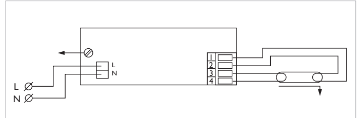
HF BALLAST
